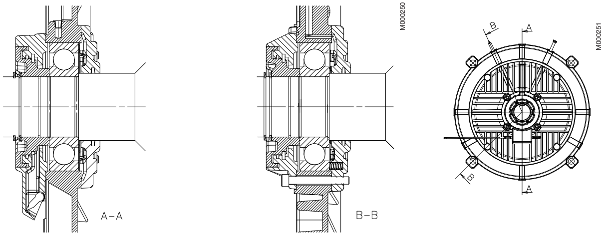
Axially free (N-end)
