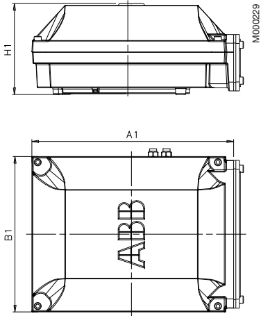
Side-mounted Terminal box 750
