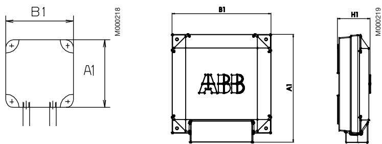
Motor sizes 71 - 132
