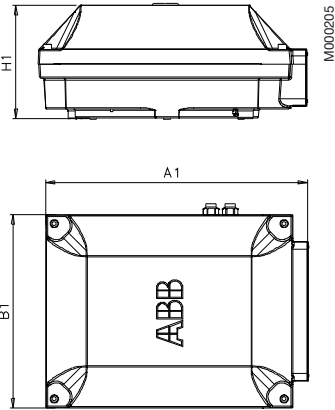
Motor sizes 280-315 Top- and side-mounted Terminal boxes 210, 370
