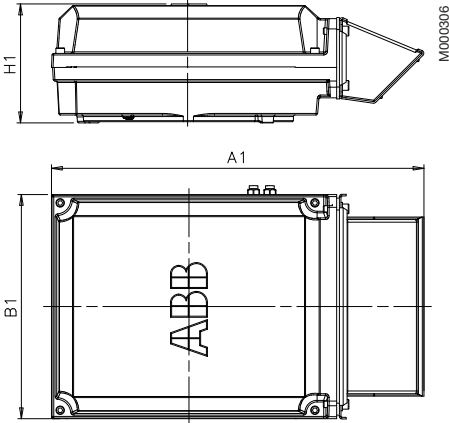
Motor sizes 355-450 Top-mounted Terminal box 750 + adapter
