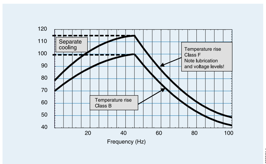
Figure 3. Motor loadability with ACS 800, Field weakening point 50 Hz.
