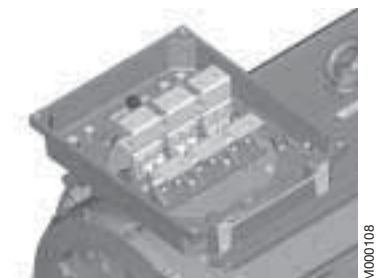
Terminal box for motor sizes 355 to 450, provided either with a cable gland or a cable box.
