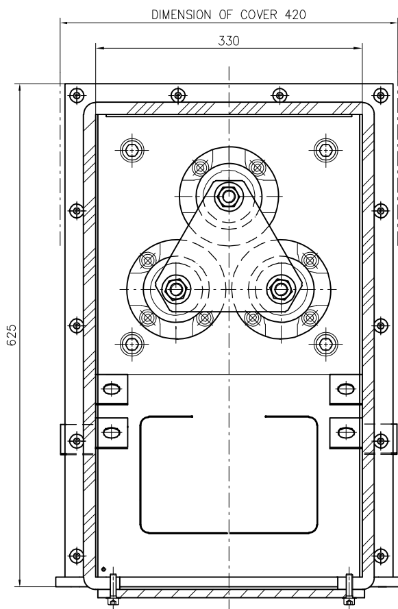
High voltage star point terminal box up to 6.6 kV.
