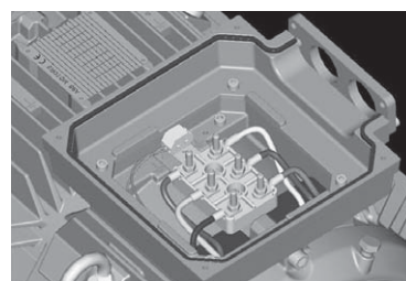
Terminal box for motor sizes 160 to 250
