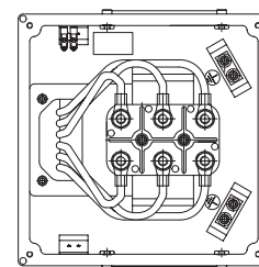
Terminal box size 200-280, except M2AA 200.
