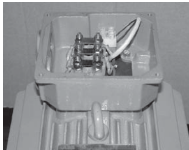
Terminal box for motors M2QA 71 to 132
