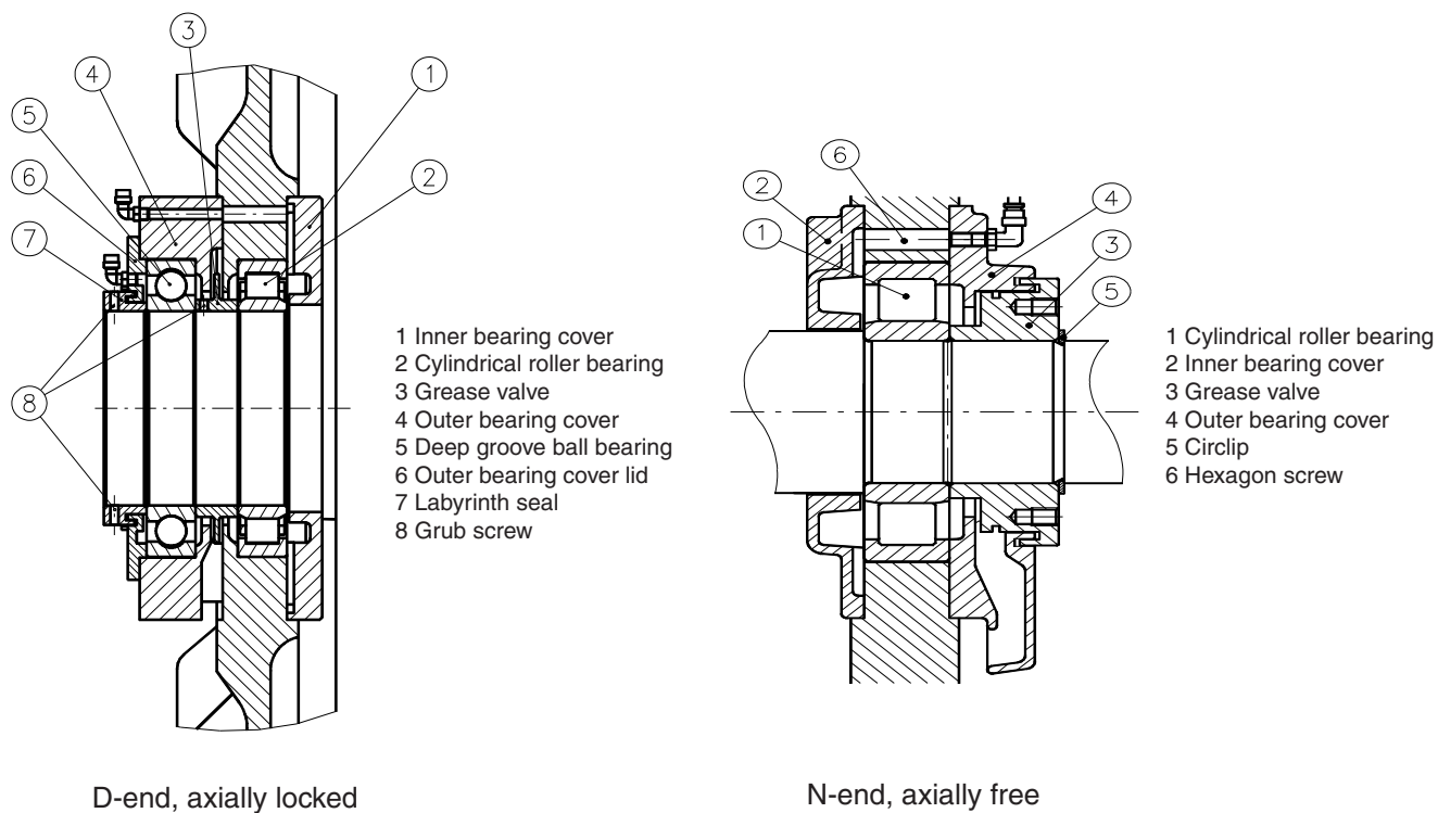
Figure below: Standard bearing construction for horizontally mounted motors HXR 560.
