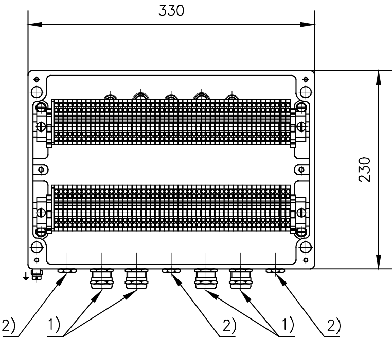
Standard terminal box ZWA ALX233318 with terminal blocks and cable glands. 1) Cable gland M20x1.5 for cable outer diameter 10...14 mm (4 pcs) 2) Threaded hole for cable gland M16x1.5 (3 pcs), plugged.
