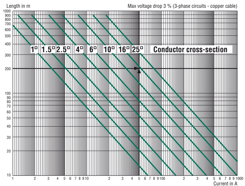
Chart 1. - Cross-section of power cables as a function of length and current carried
