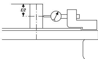
① Eccentricity of shaft in flanged motors
