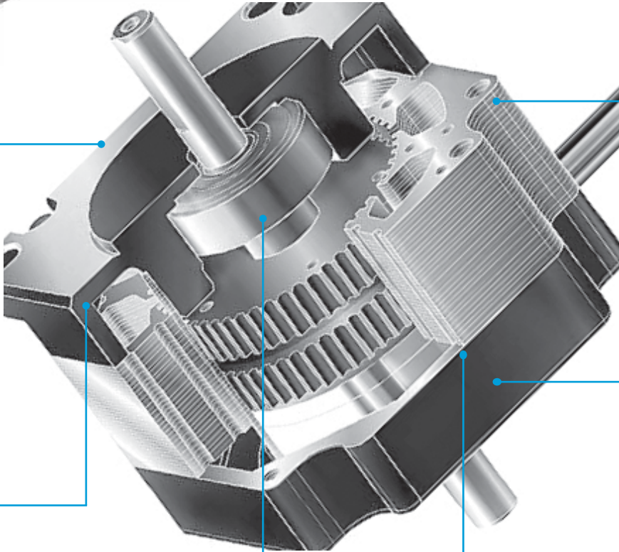
Shaft
