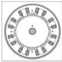
Fig. 3 - Cross-section of a hybrid stepper motor.
